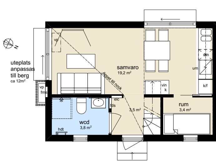
Plan bv
